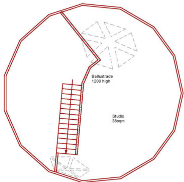
30ft Dome Second Floor Plan
