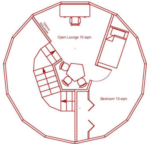
24ft Dome Second Floor Plan
