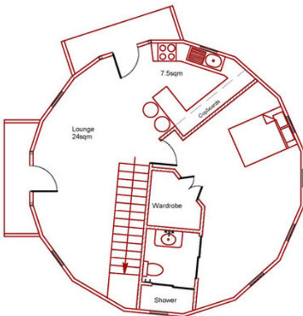
30ft Dome First Floor Plan
