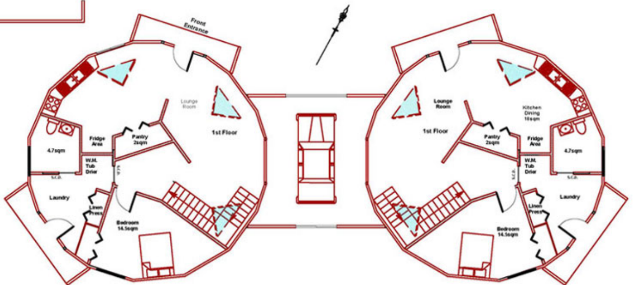
35ft Dome Duplex First Floor Plan
