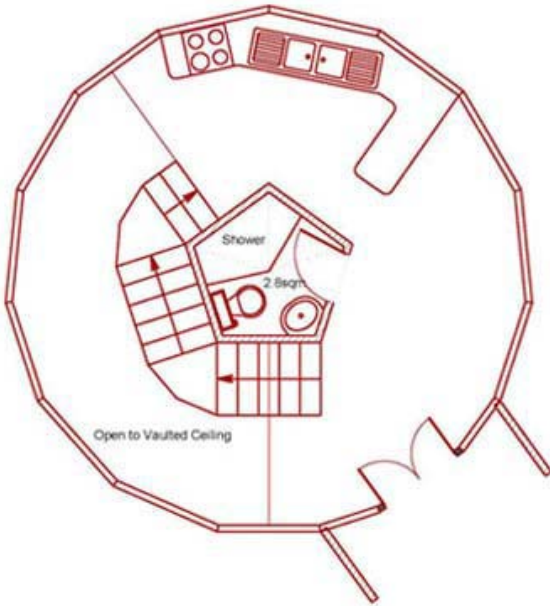
24ft Dome First Floor Plan
