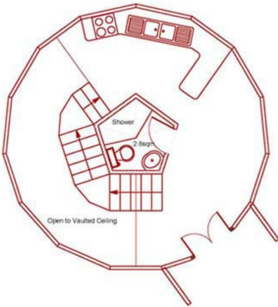
24ft Dome First Floor Plan
